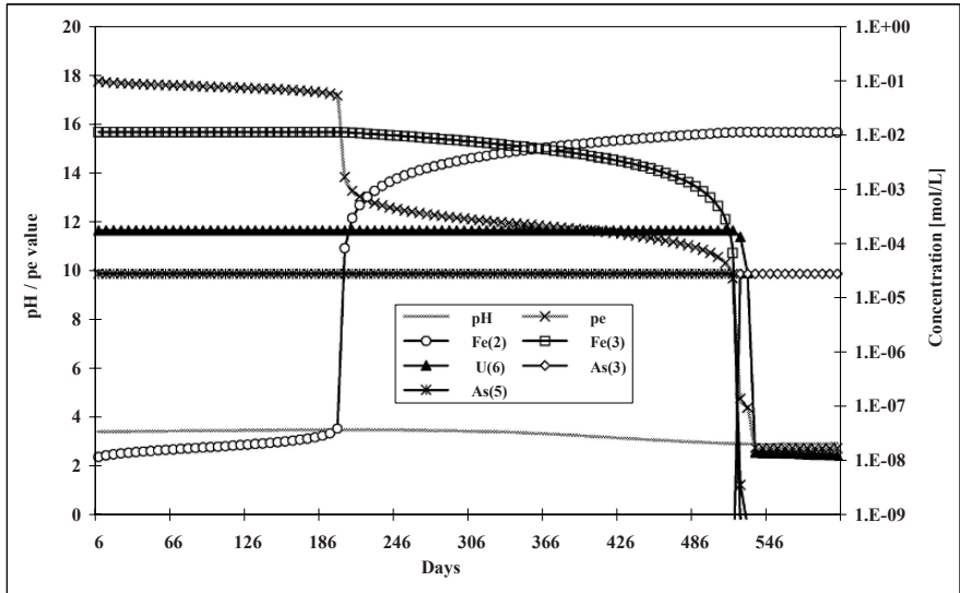
Fig. 85 Changes in the speciation of iron, arsenic, and uranium compared to pE and pH values during the degradation of organic matter over a period of 600 days
