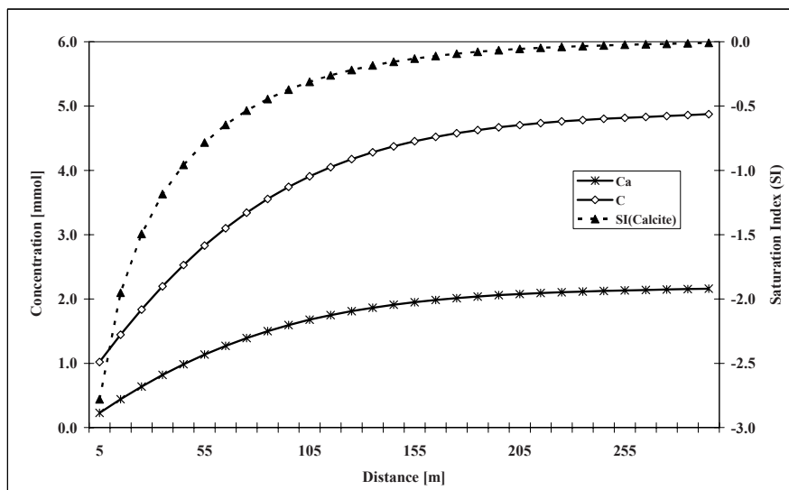
Fig. 89 Corrosion in a fracture showing convergence to the calcite equilibrium with increasing distance
