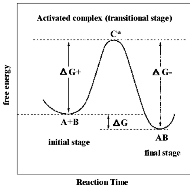
Fig. 25 Scheme of the free energies \Delta G and formation of an activated complex C^* as a transitional state of the reaction A+B=AB (after Langmuir 1997)
