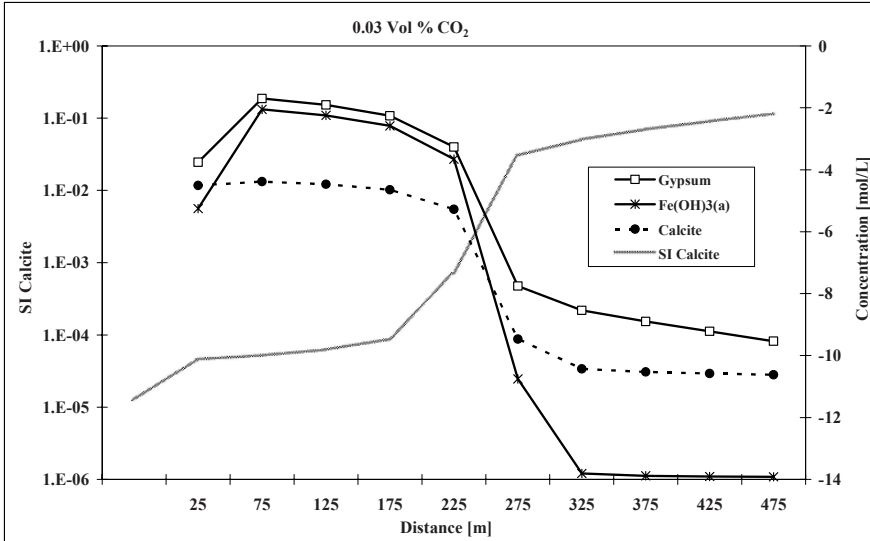
Fig. 91 Dissolution of calcite, precipitation of gypsum and iron hydroxides, and the development of the calcite saturation index for the AMD water shown in Fig. 90
