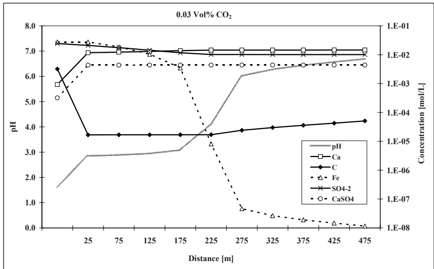
Fig. 90 Concentration changes in an acid mine water while flowing through a 500 m long carbonate channel
