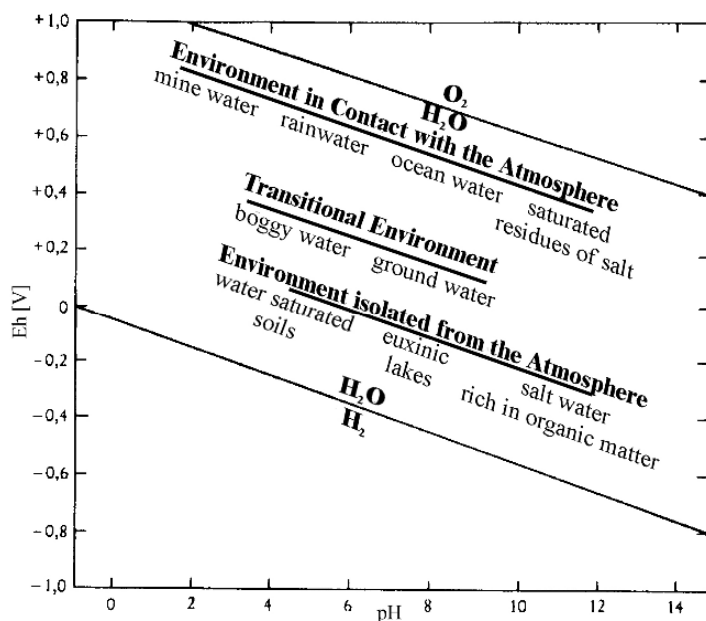
Fig. 17 Classification of natural waters under various E H /pH conditions (modified after Wedepohl 1978)
