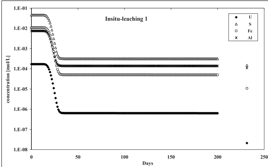
Fig. 92 Simulated concentration at the pumping well over a period of 200 days (fracture volume 0.05, pore volume 0.15, 10 cm of pore matrix connected to the fracture), points on the right side mark the target concentrations.
