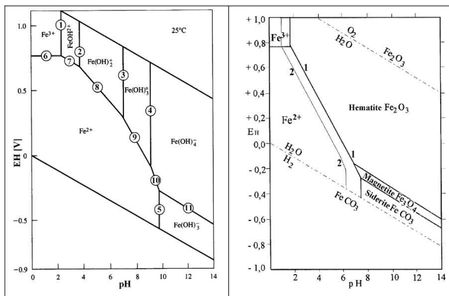
Fig. 16 Left: E_H -pH diagram for the system Fe-O 2 -H 2 O (at 25°C, the numbers 1-11 correspond to the reaction equations described in the text for the calculation of the stability fields, modified after Langmuir 1997) Right: E_H -pH diagram for the system Fe-O 2 -H 2 O-CO 2 (at 25°C, P(\text{CO}_2) = 10^{-2} atm), for fields where the total activity is < 10^{-6} (1) resp. < 10^{-4} (2) mol/L the predominant, precipitating mineral phase is outlined (modified after Garrels and Christ 1965).
