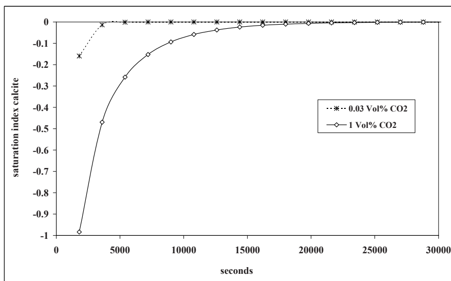
Fig. 45 Time-dependent calcite dissolution at 0.03 Vol% CO 2 (atmospheric pressure) and increased CO 2 partial pressure (1 Vol%)
