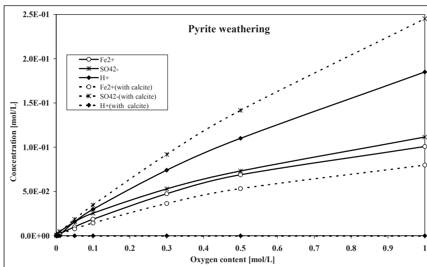
Fig. 68 Effects of pyrite weathering on the concentrations of \text{Fe}^{2+} , \text{SO}_4^{2-} and \text{H}^+ in the absence and in the presence of calcite
