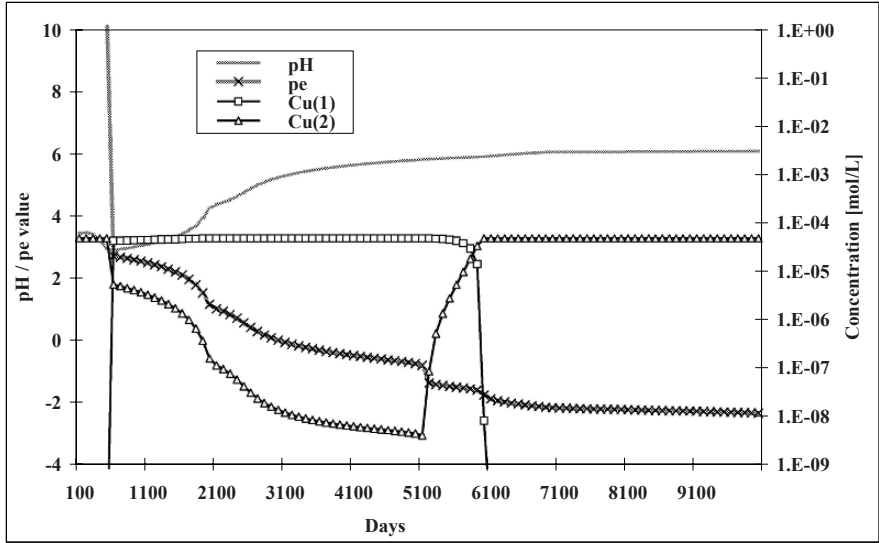
Fig. 84 Changes in the speciation of \text{Cu}^+ and \text{Cu}^{2+} in relation to pE and pH values during the degradation of organic matter over a period of 10,000 days
