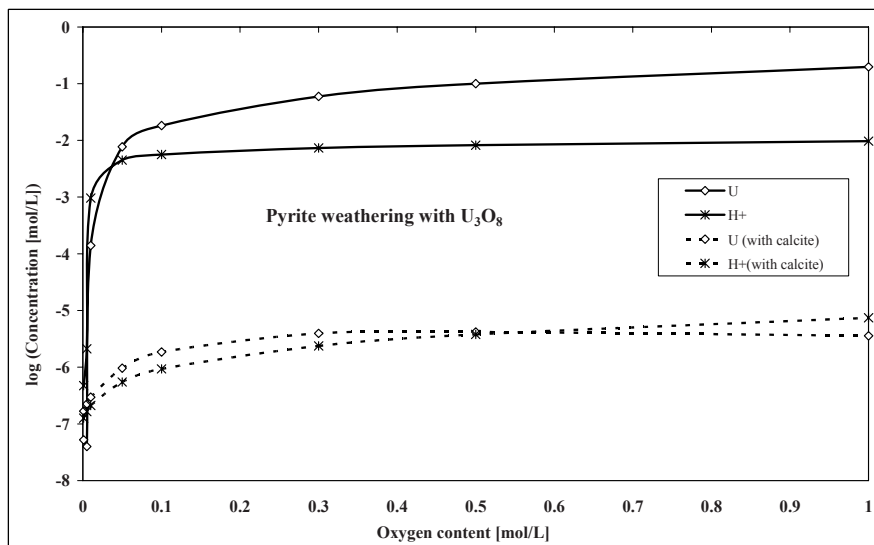
Fig. 69 Effects of pyrite weathering in the presence of the mineral phase \text{U}_3\text{O}_8 on the concentrations of uranium and \text{H}^+ in the absence and in the presence of calcite (y-axis logarithmic).
