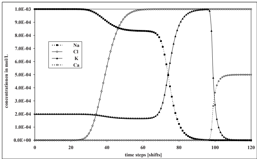
Fig. 48 Laboratory column experiment: changes in chloride, sodium, potassium, and calcium concentrations at the column’s outlet; 40 “shifts” correspond to a complete exchange of the water volume within the column
