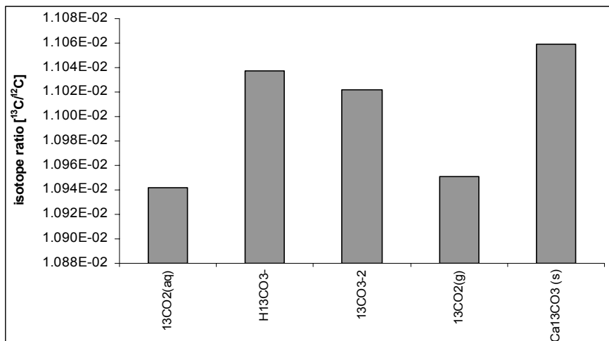
Fig. 46 Calculated \delta^{13}\text{C} C-values at 25°C in the three phases gas ( \text{CO}_2 ), water, and mineral (calcite)
